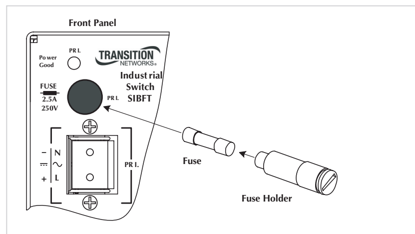
Figure 15: Fuse Replacement
